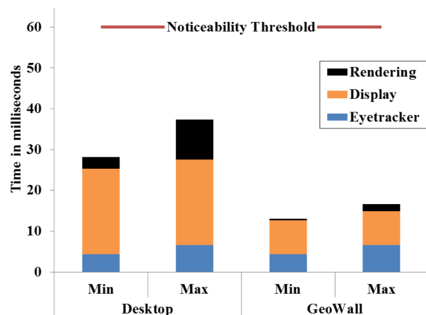
Figure 2: In Desktop and GeoWall setups, the minimum and maximum computation time required by the GeoGCD (for rendering, displaying, and eye tracking) remain below the 60ms noticeability threshold reported in Loschky and Wolverton [2007] and Albert et al. [2017].
