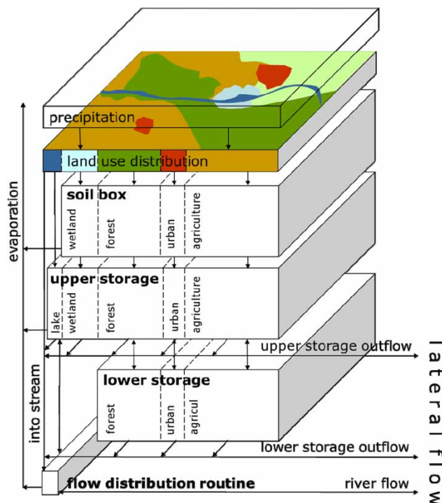
Figure 2 | Schematic representation of the sub-grid parameterization scheme in a single model grid cell. All water flows and storages within the model routines are weighted according to their designated land use class. Vertical flows indicate fluxes between different model storage compartments. Lateral flows indicate fluxes to neighbouring draining grid cells.
